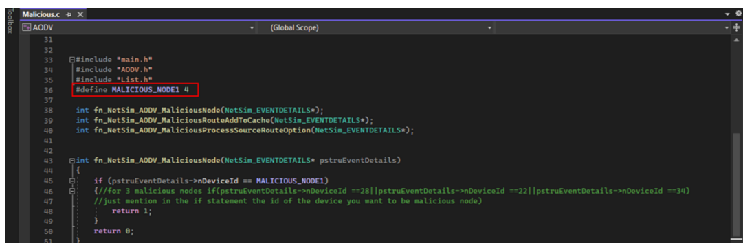
Figure 2-1: Set malicious node in the malicious.c file.
