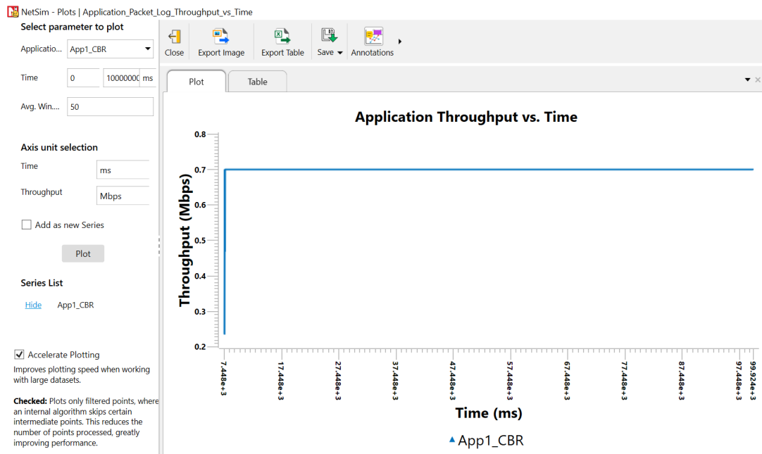
Figure 3-2: Initially, all traffic flows to the malicious node, resulting in a zero throughput until approximately 7.38 seconds. Upon detection of the malicious activity and subsequent rerouting of traffic, the throughput shows a significant increase, indicating the normal data flow.
