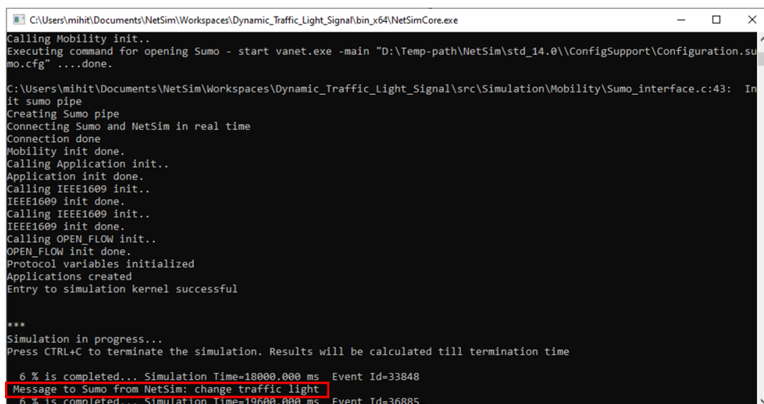
Figure 6-2: Control message being sent from NetSim to Sumo.
