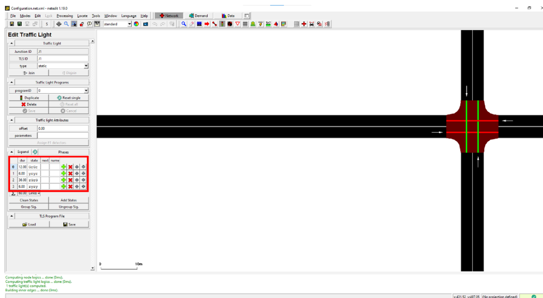
Figure 4-1: Four phases of traffic signal defined in sumo.
