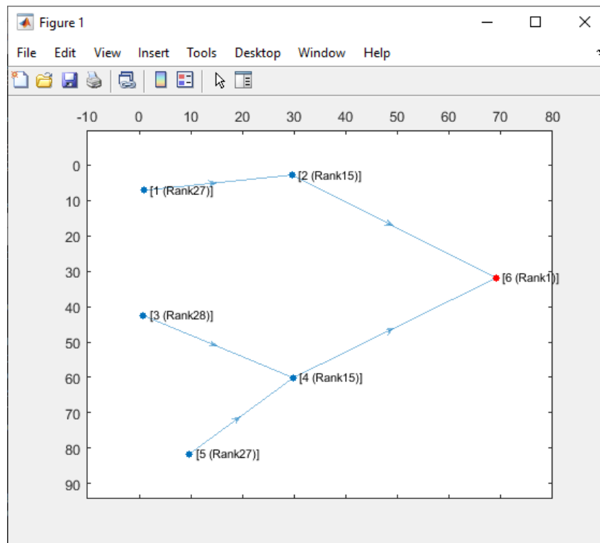
Figure 3: Plot of DODAG Formation in MATLAB
