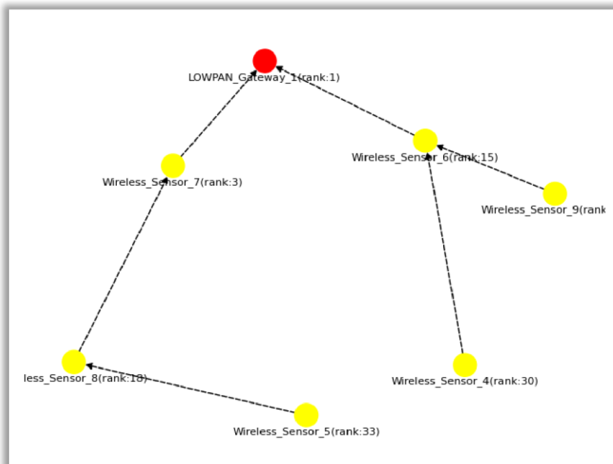
Figure 9: RPL DODAG Visualizer
