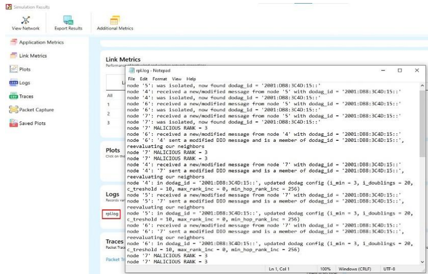
Figure 3: Result Dashboard Window
