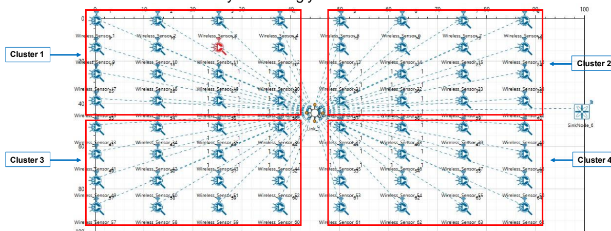
Figure 8: Sensor nodes present in each Clusters
