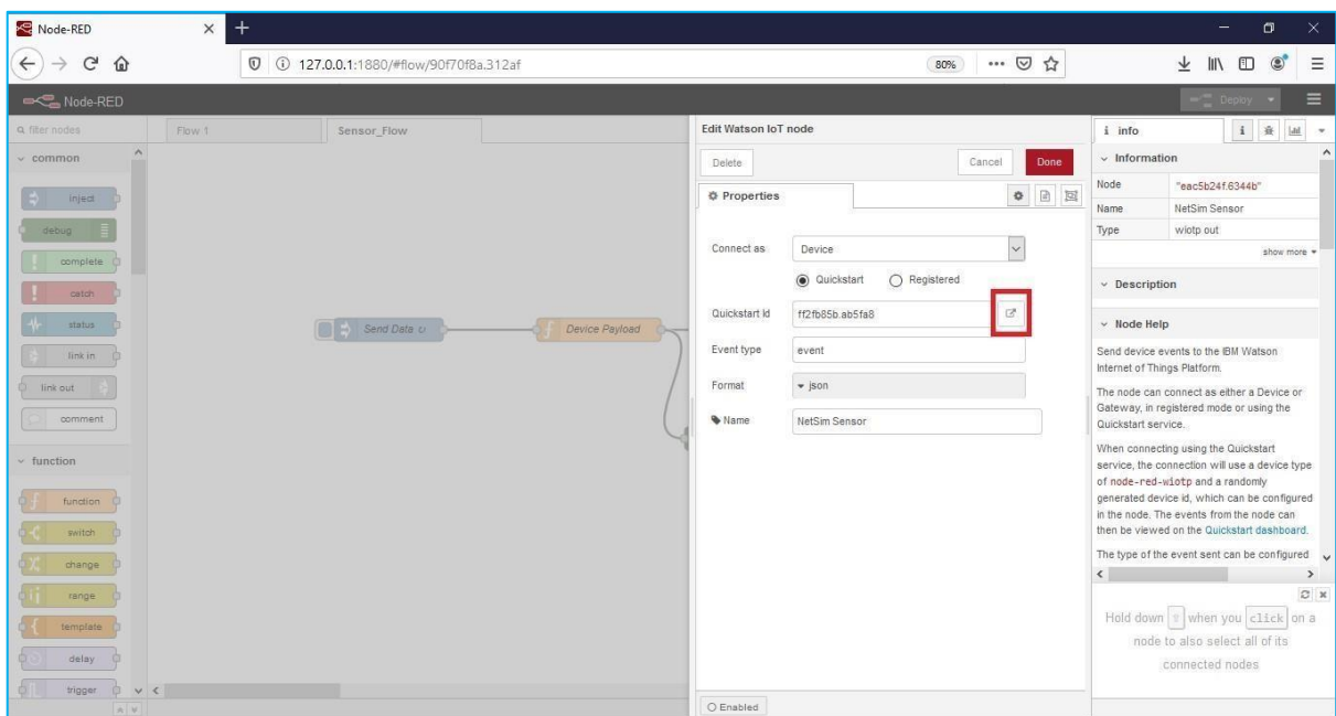
Figure 4: Quickstart Id set in Blue NetSim Sensor icon
