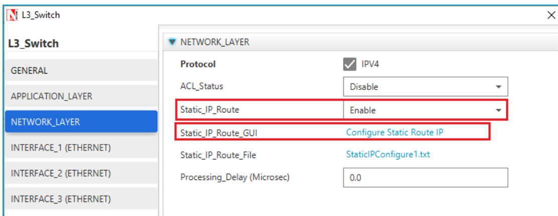
Figure 30-7: Select Configure Static Route IP
