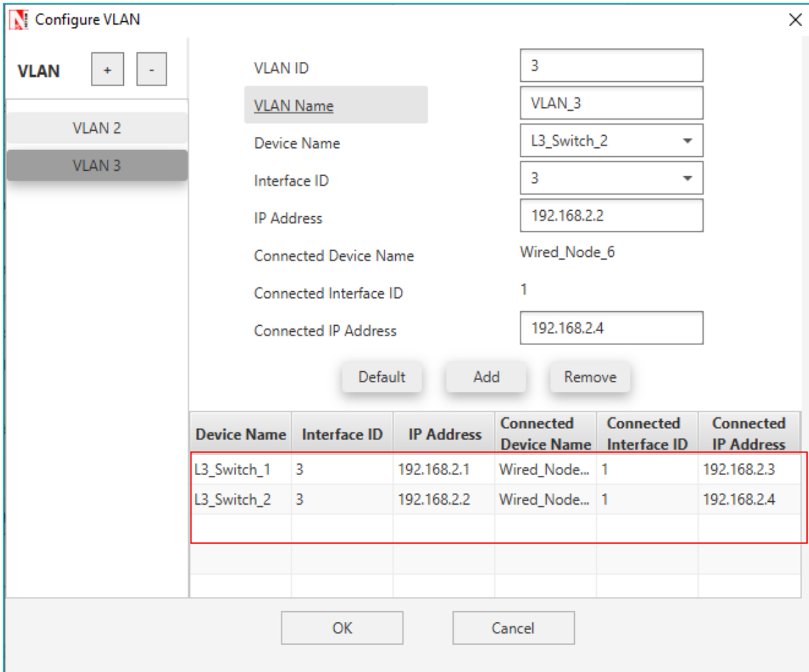
Figure 30-6: Configuring VLAN Properties in VLAN 3
