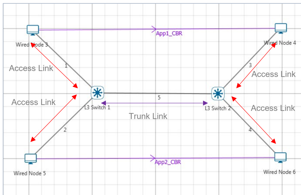
Figure 30-1: Understanding Access and Trunk Links in VLANs
