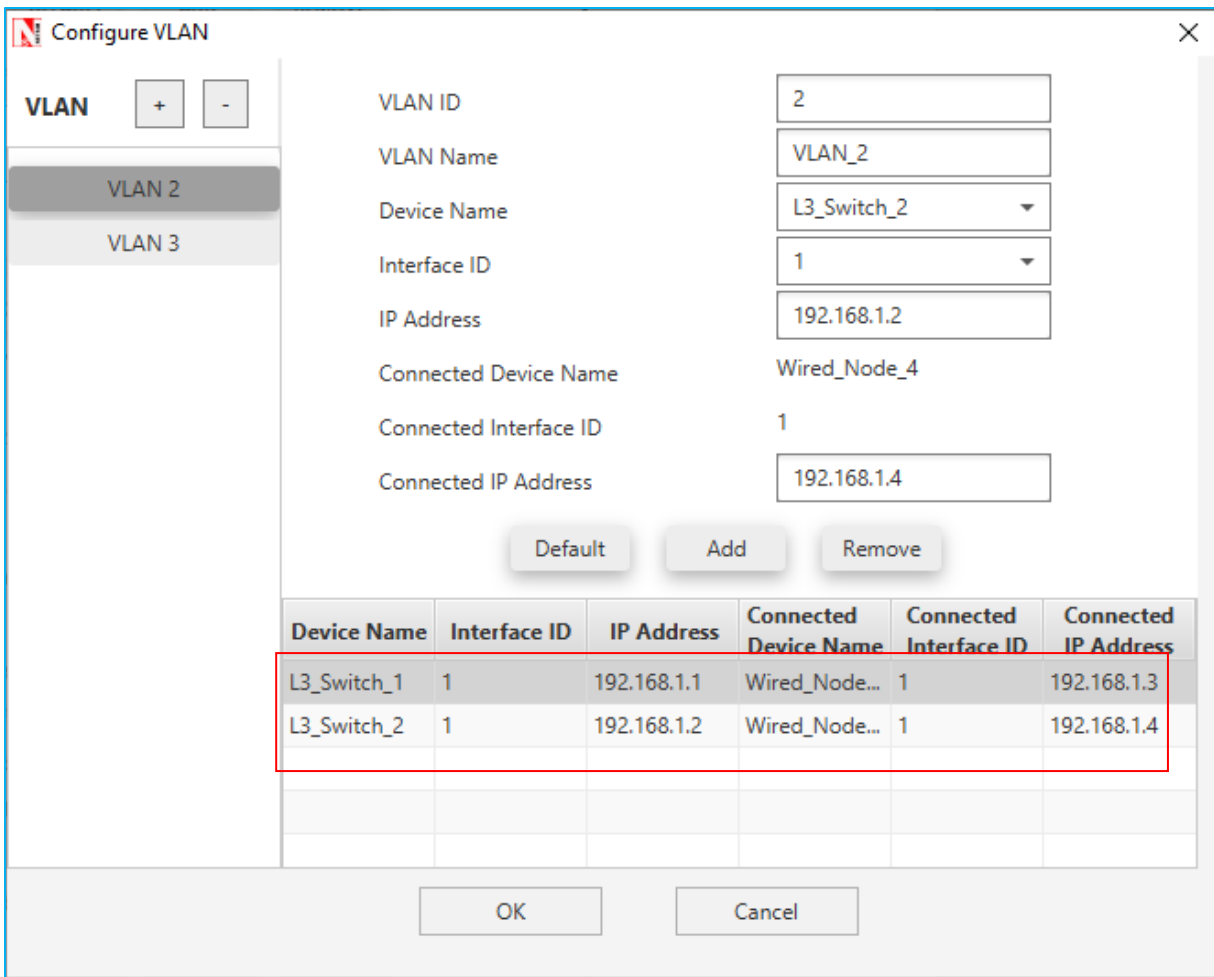
Figure 30-5: Configuring VLAN Properties in VLAN 2
