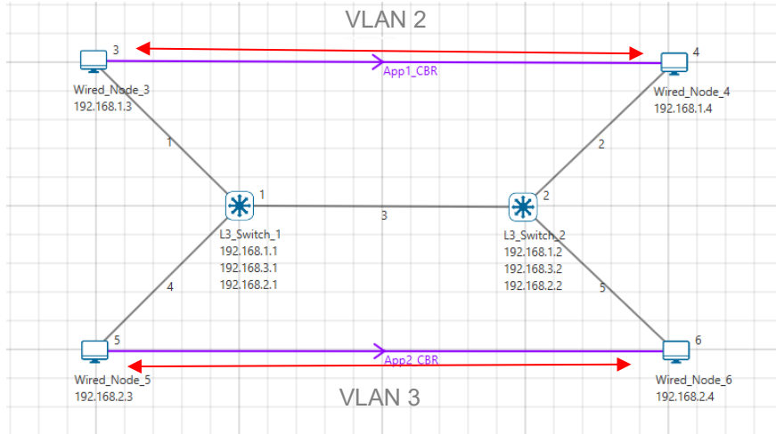
Figure 30-3: Network Topology in this experiment
