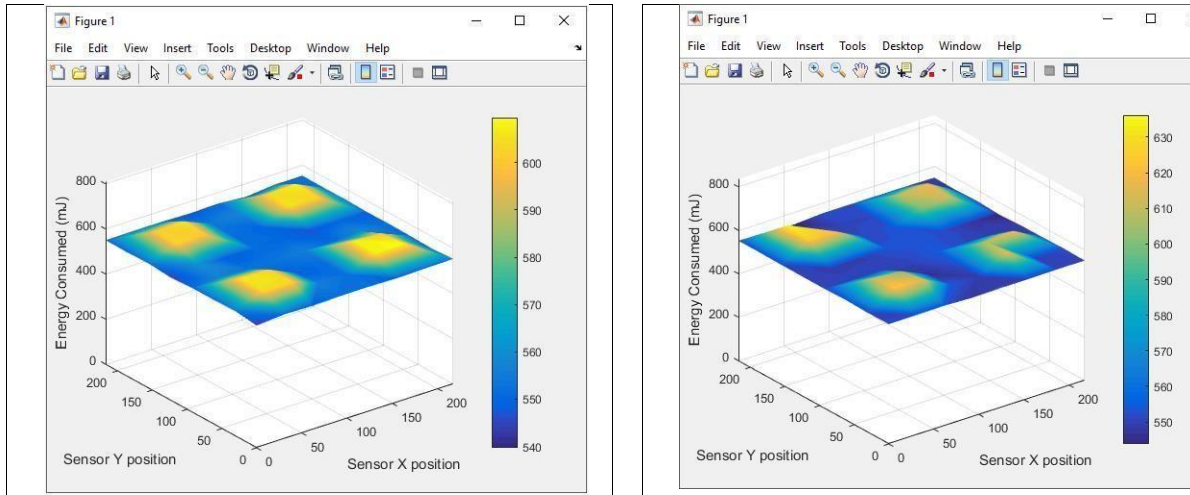
Figure 5: Energy consumption plots for k means and fuzzy c-means algorithms using method 3 and 4. In the initial phase the plot resembles the previous one. However, as time passes, it can be observed that the power is consumed by all the sensors at approximately the same rate.
