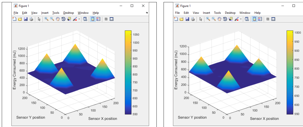
Figure 4: Energy consumption plots for k means and fuzzy c-means algorithms using methods 1 and 2. As it is seen from the plot, there are 4 peaks in the plot corresponding to higher energy consumption in the nodes in the center of the cluster, as they always become the cluster heads. This is because the distance is used as a parameter for electing the cluster heads.
