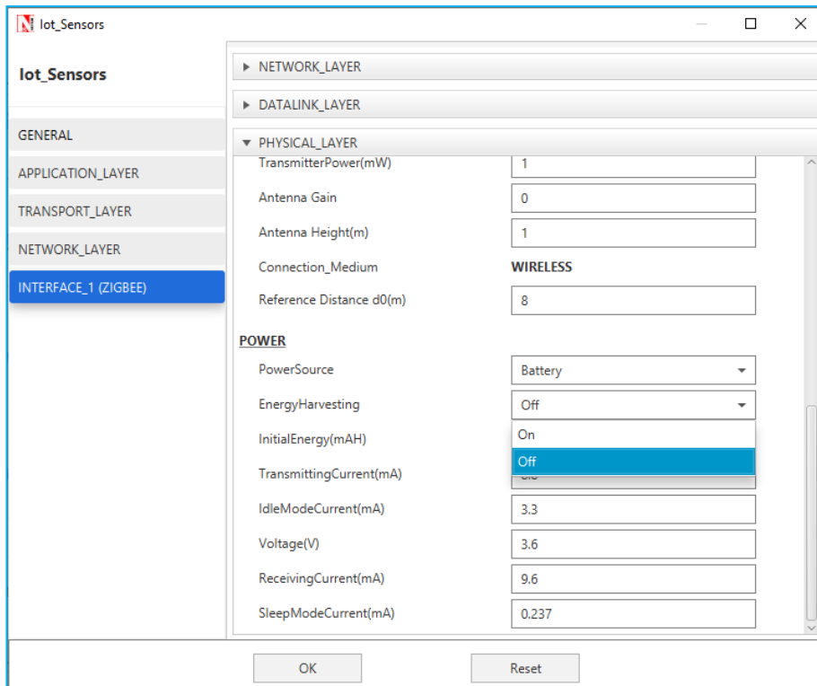
Figure 3: Disable Energy Harvesting in all Sensor nodes
