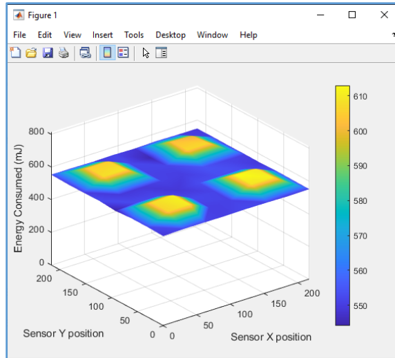
Figure 10: Plot for Power Consumption of Sensors
