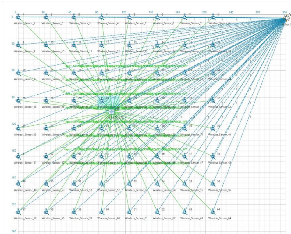
Figure 3: Network Topology
