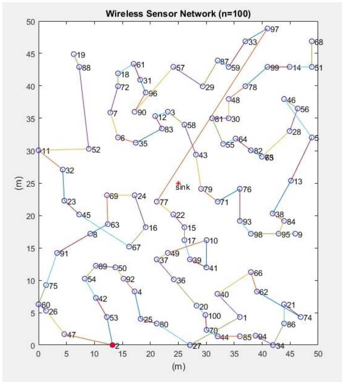
Figure 5: Nodes that are part of the network in NetSim Shown in MATLAB
