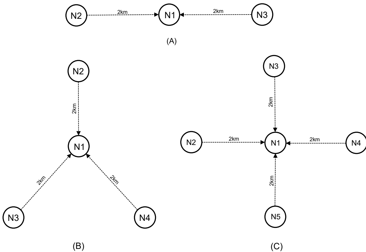
Figure 4-5: Simulation scenarios with 2 transmitting nodes in (A), 3 transmitting nodes in (B) and 4 transmitting nodes in (C). In all cases there is a single receiver.
