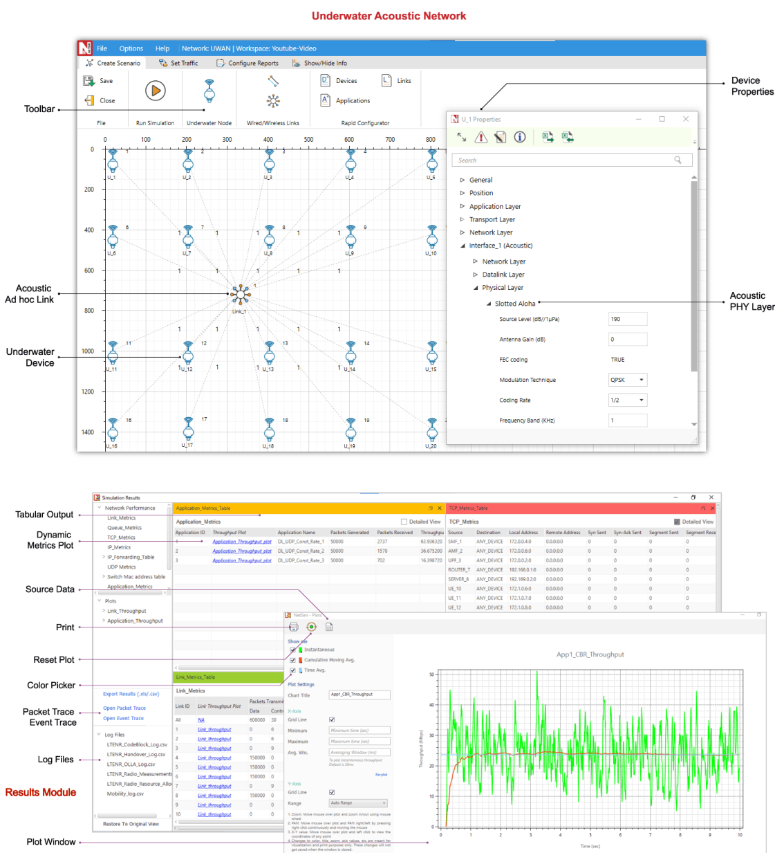
Figure 1-1: NetSim's UWAN design window, the results dashboard, and the plots window
