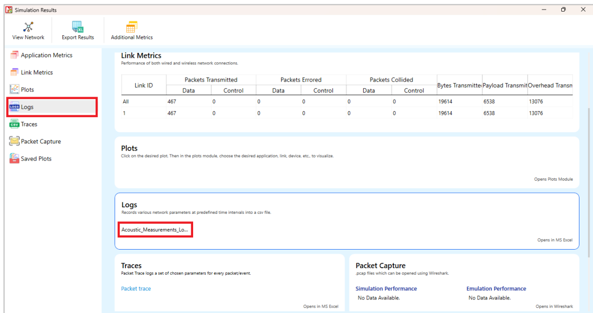
Figure 3-2: Acoustic_Measurements_Log.csv file highlighted in the Results window.
